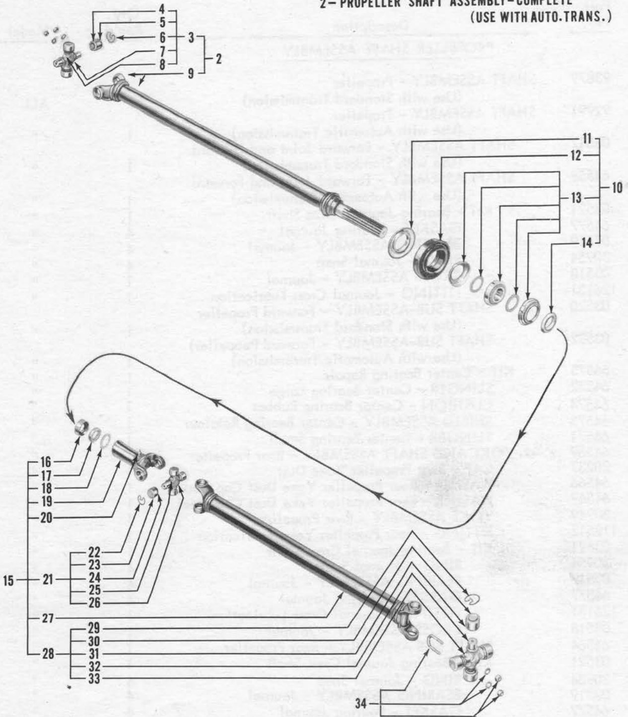
PROPELLER SHAFT ASSEMBLY ILLUSTRATION NO. 39
