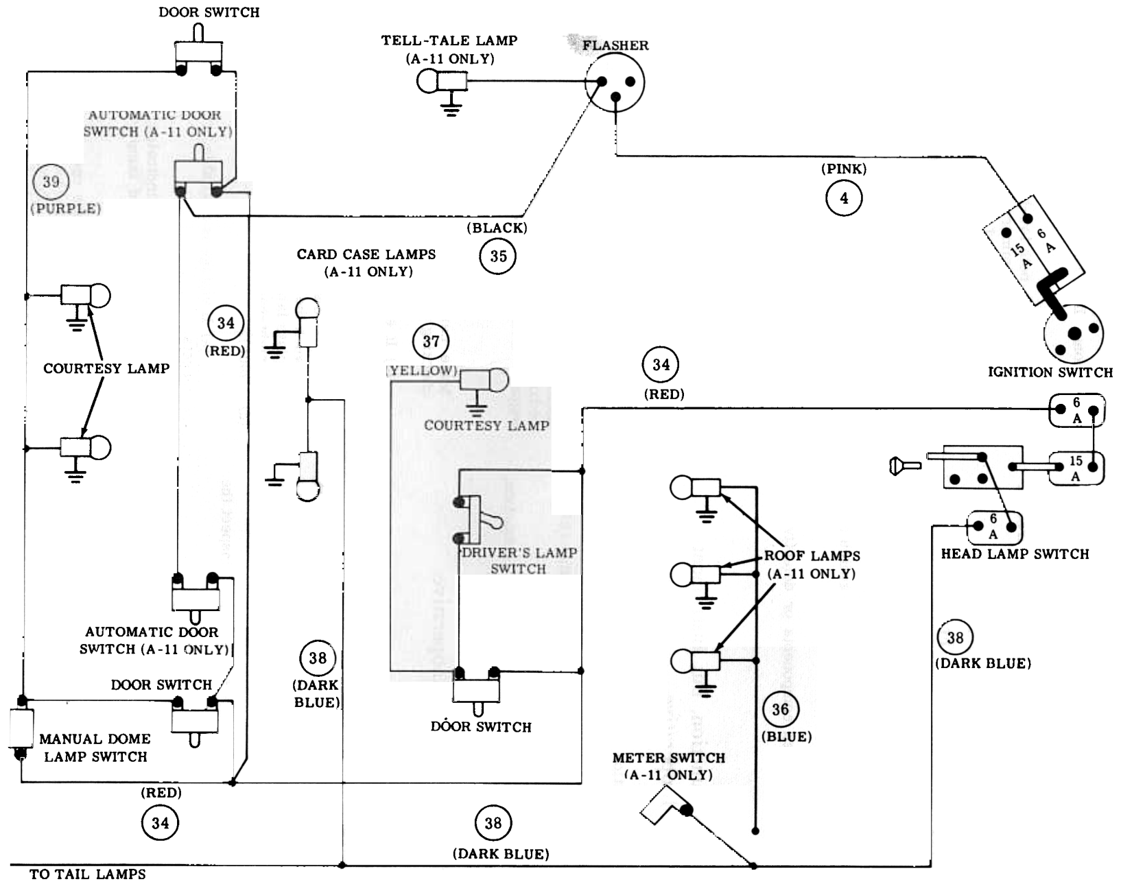
Fig. 3 - Internal Lamp Wiring
