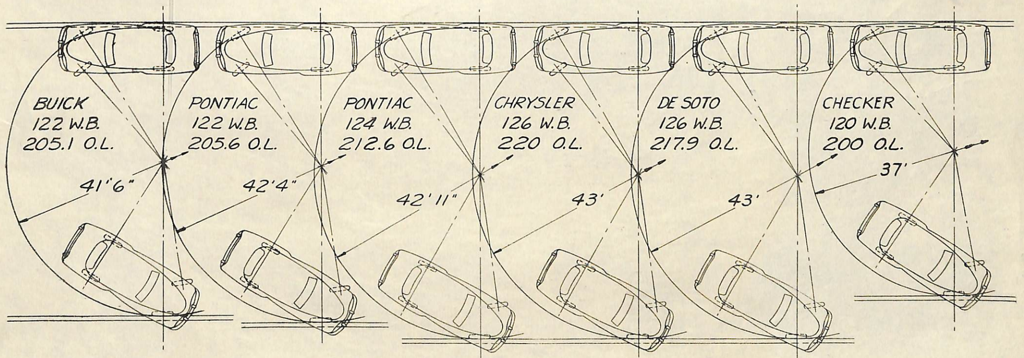
TURNING CIRCLE DIAMETERS 1956 CARS
